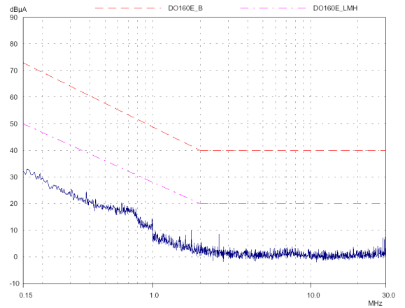
D0-160E : MGDS-75-0-C with FGDS-10A-50V
