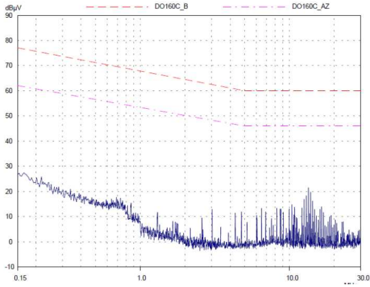
DO-160C : MGDS-75-H-F with FGDS-10A-50V
