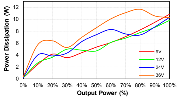
CEB100W-24S54 Pd Vs Po @25 Deg. C
