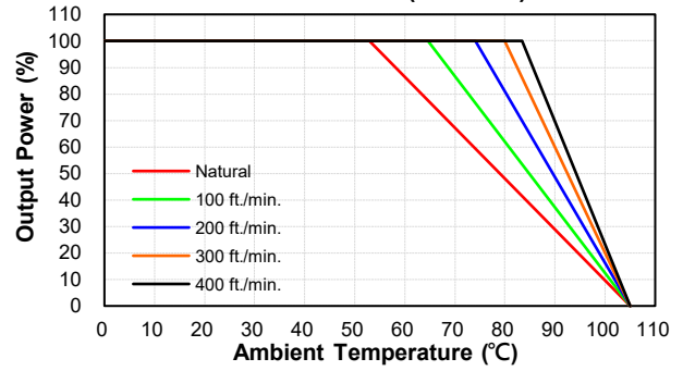
CEB100W-24S12, 48 Derating Curve with Heatsink (Vin=24V)
