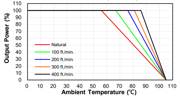
CEB100W-24S05, 54 Derating Curve with Heatsink (Vin=24V)
