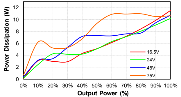
CEB100W-48S24 Pd Vs Po @25 Deg. C
