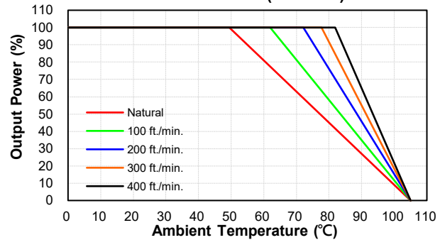
CEB100W-24S24 Derating Curve with Heatsink (Vin=24V)
