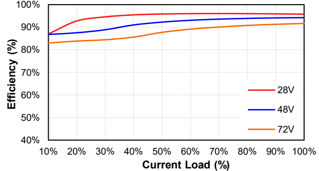
NCS01W8-48S240 Eff Vs Io @25 Deg. C
